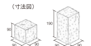
■ EK1251 1丁掛 ■ EK2241 2丁掛
